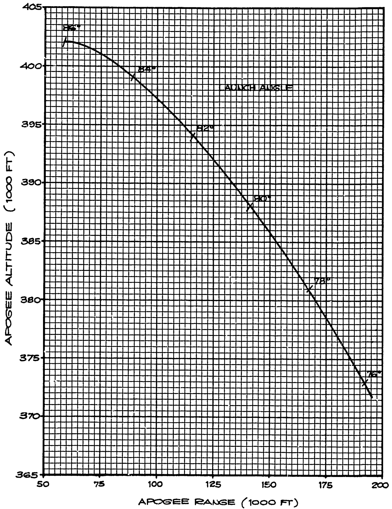
FIGURE 6 VIPER IIIA DART APOGEE PERFORMANCE
