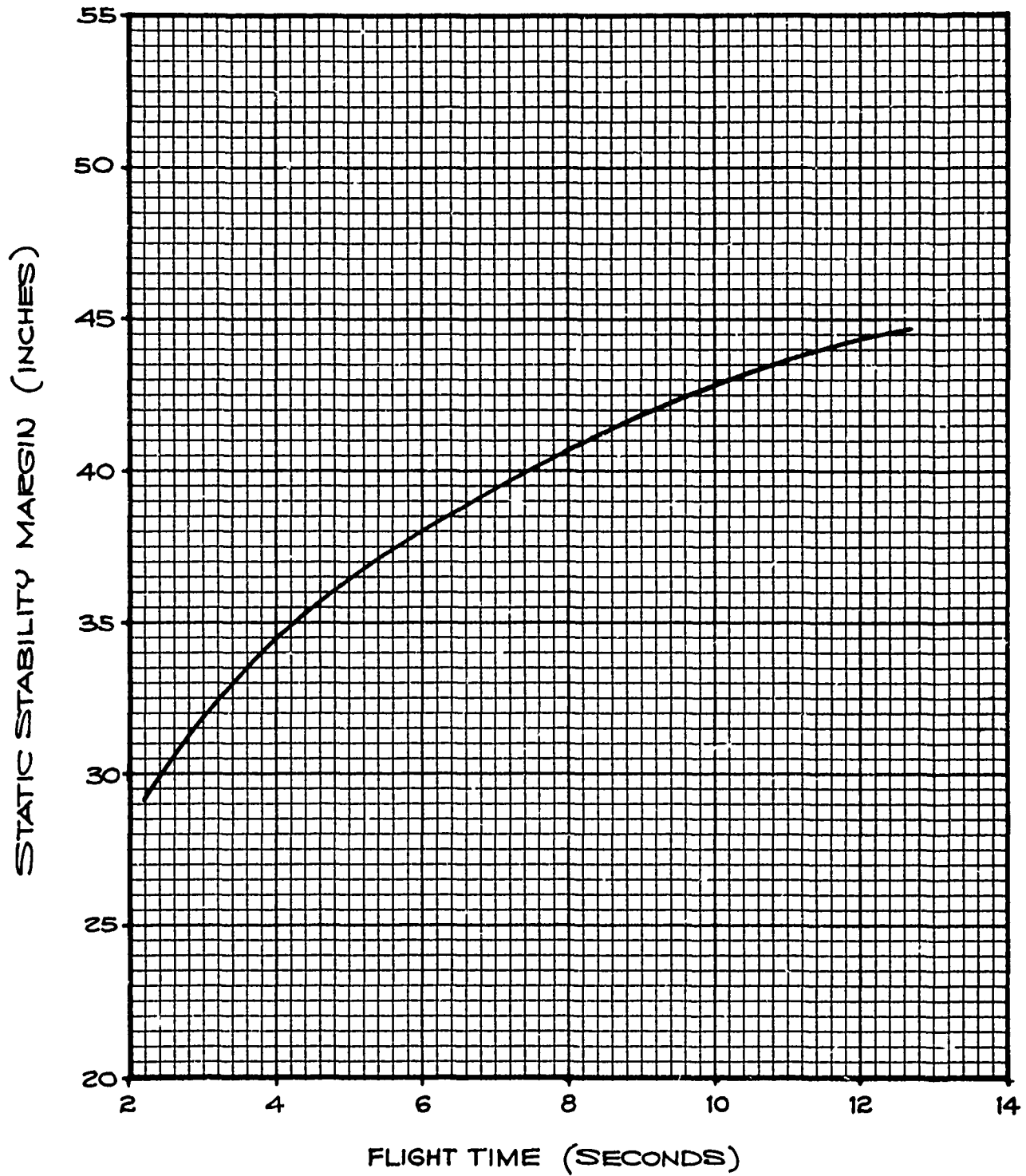
FIGURE 5 EXPENDED BOOSTER STATIC STABILITY MARGIN
