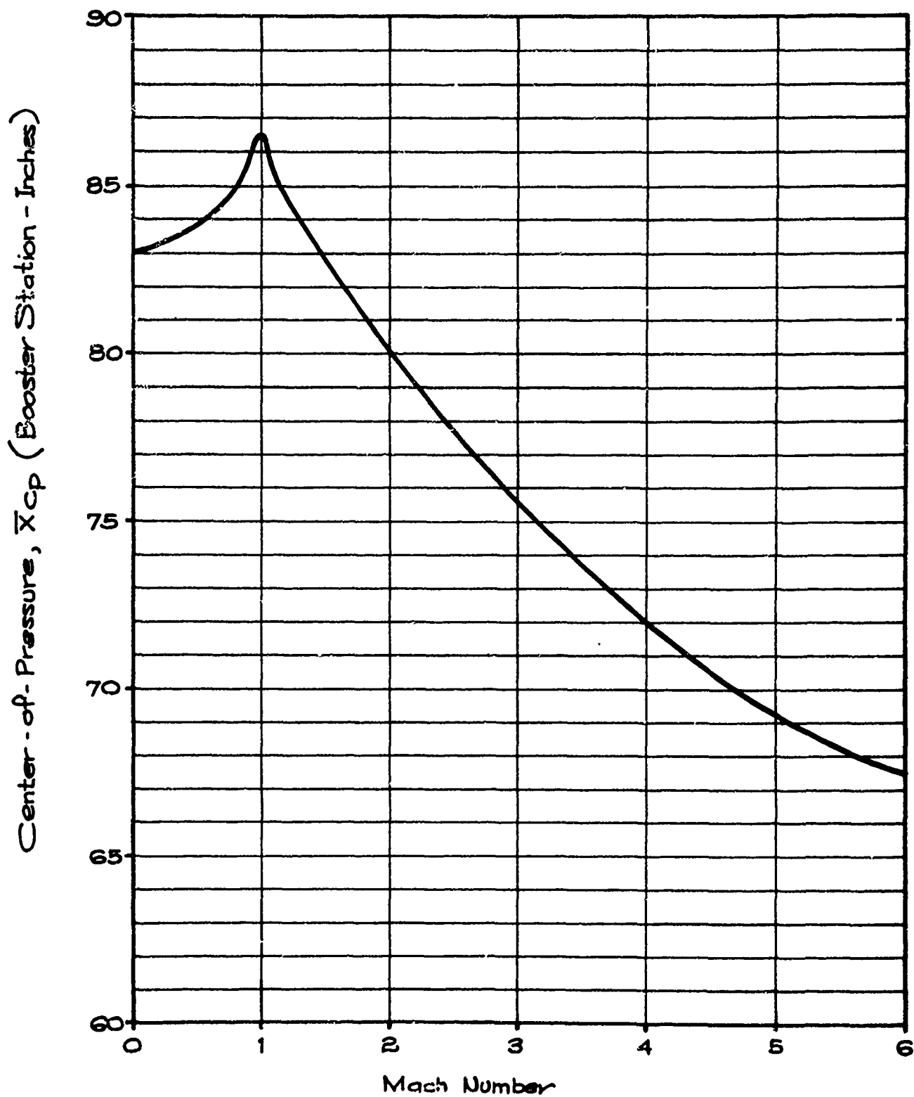
FIGURE 7.3 EXPENDED STABLE SUPER LOKI BOOSTER CENTER-OF-PRESSURE
