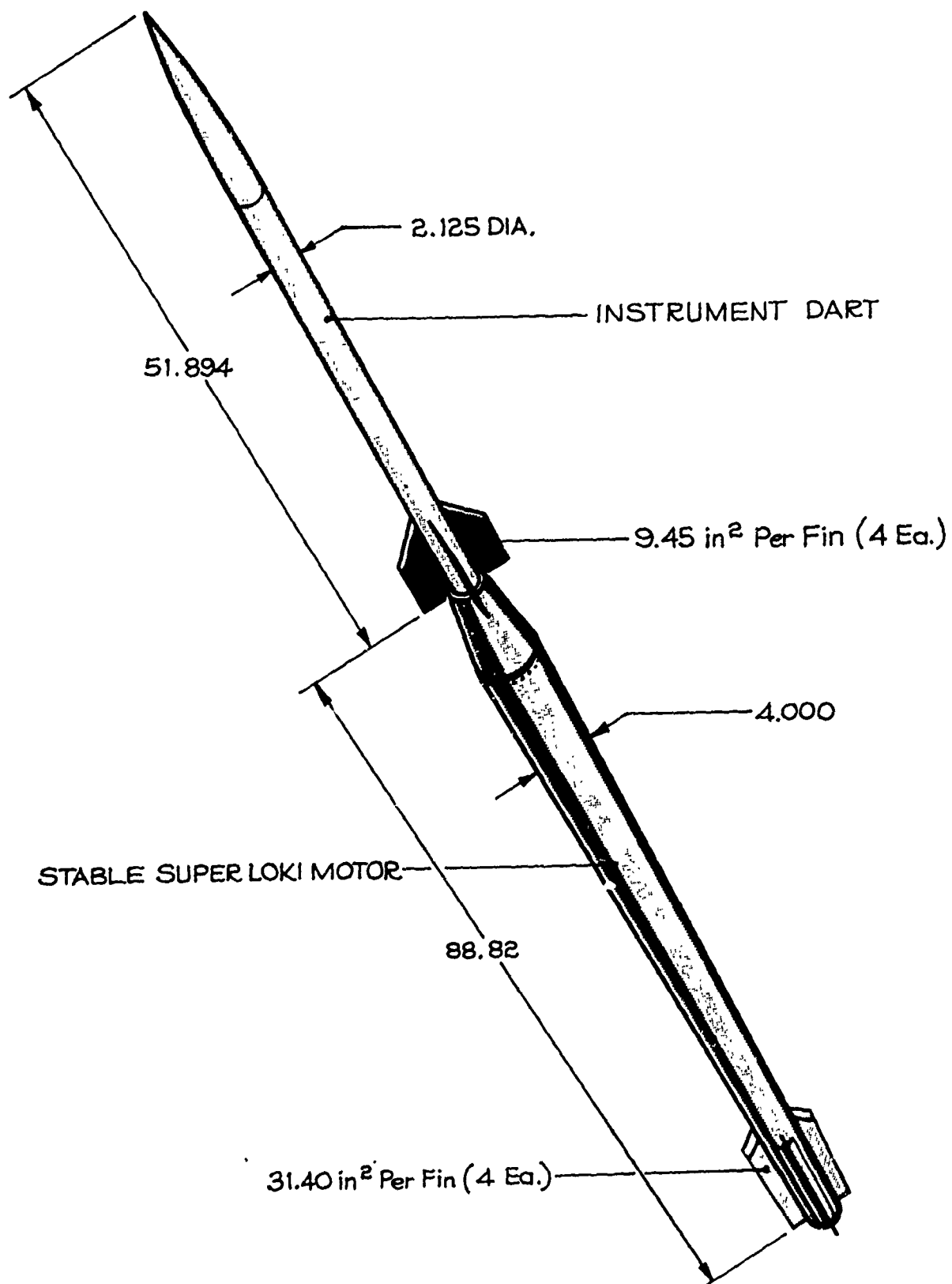
FIGURE 5.1 STABLE SUPER LOKI INSTRUMENT DART VEHICLE CONFIGURATION
