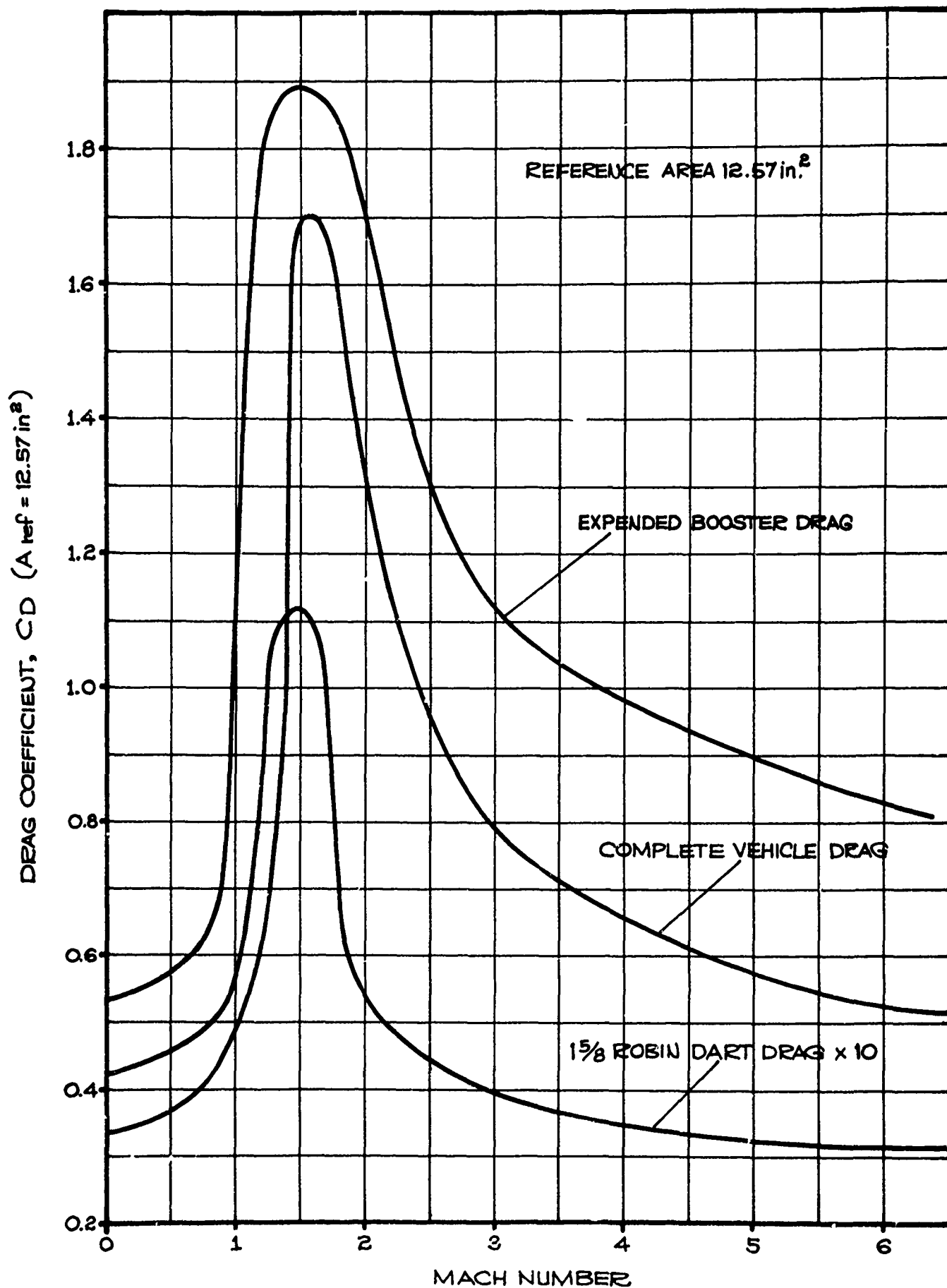
FIGURE 4.8 STABLE SUPER LOKI ROBIN VEHICLE DRAG COEFFICIENTS
