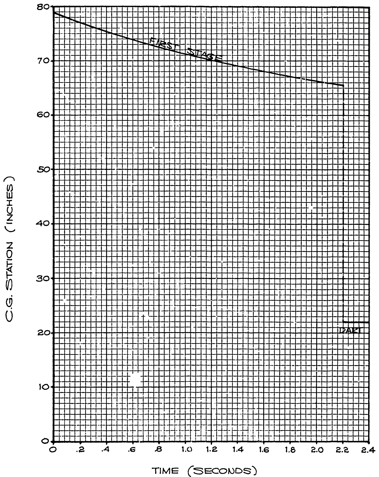
FIGURE 1 VIPER IIIA STABLE BOOSTER DART VEHICLE 1\frac{5}{8} DART / 13.5 LB. CENTER-OF-GRAVITY
