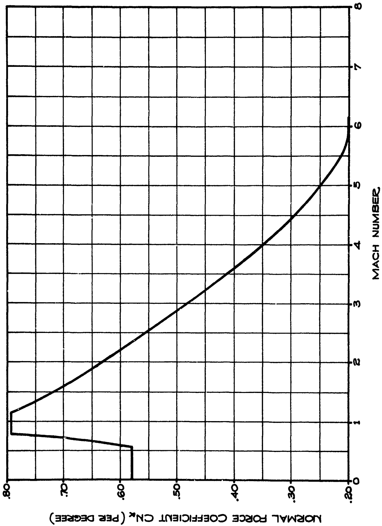
FIGURE 4.4 SUPER LOKI ROBIN DART C_{N\alpha} VS. MACH NO. FIRST STAGE (A REF 12.55 IN 2 )
