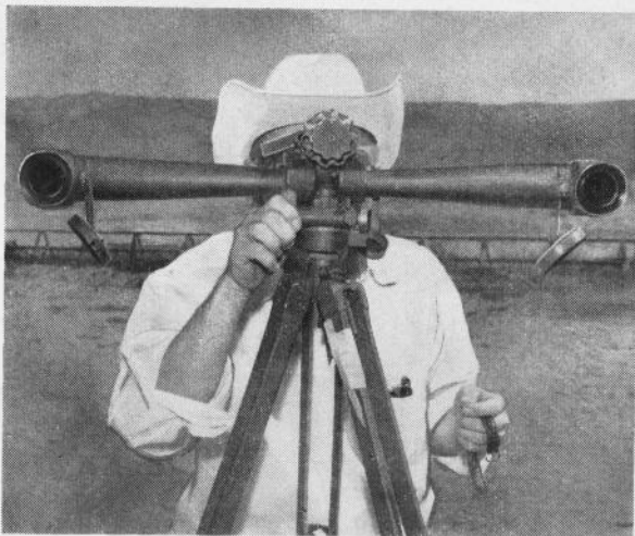
Tracking-team member sights falling rocket and records bearing. Location of the buried rocket can be found by triangulation
